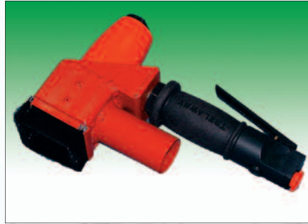
Shrouded Single Scaler including single piece Tungsten Carbide head Part No. 139.6190-Short Handle
