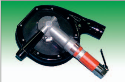
7" Air Floating Head Grinder Part No.195.5701
